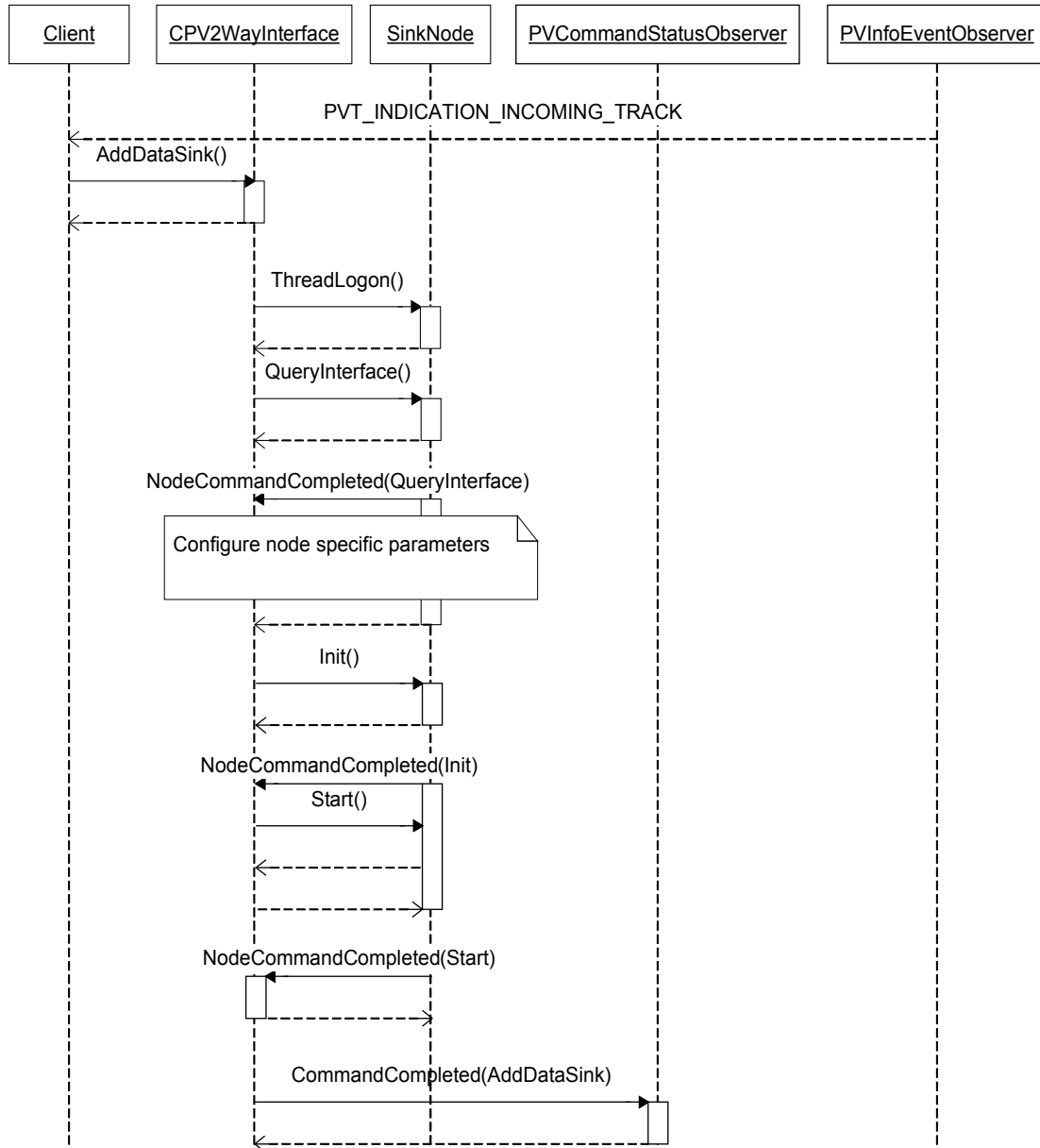
Figure 7: Sequence Diagram - Adding a Data Sink
